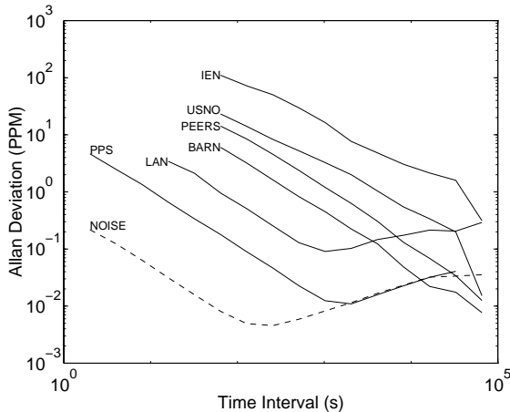
Figure 2. Allan Deviation Plot (from [MIL98])
