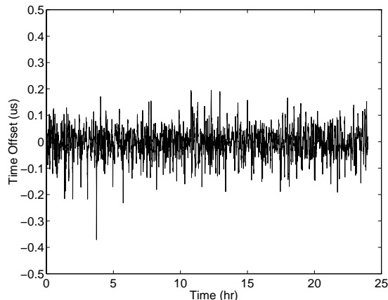
Figure 1. Nanokernel Clock Discipline with PPS Signal on Alpha 433au (from [MIL00b])
